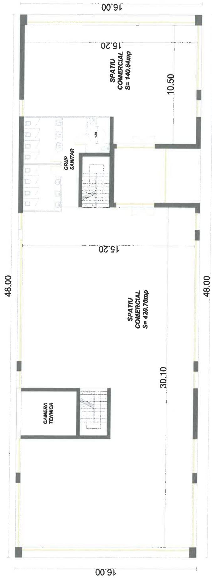
PLAN PARTER
